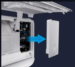
Take off PCB box cover
